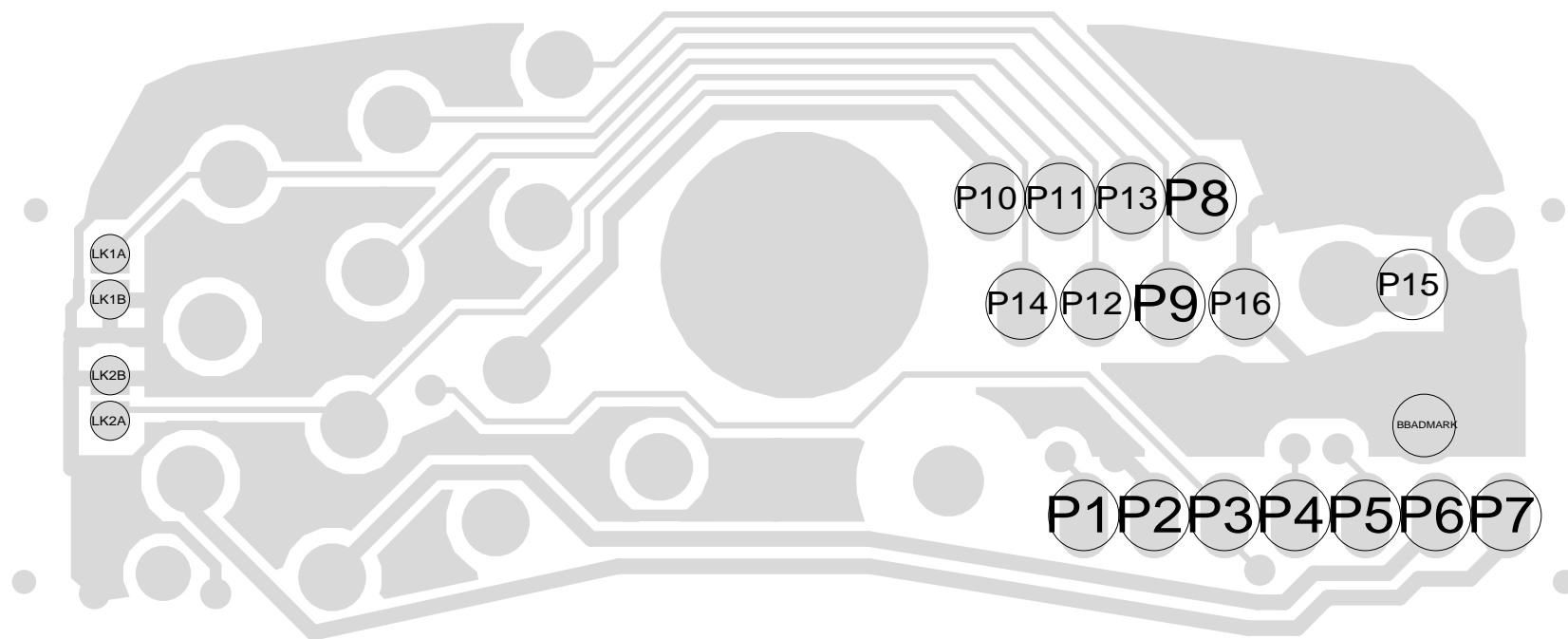
ORCA AUXILIARY CONNECTOR 220-01413-00 A BOTTOM COPPER
