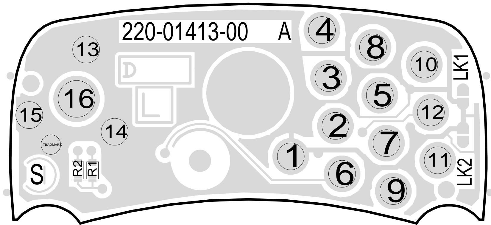
ORCA AUXILIARY CONNECTOR 220-01413-00 A TOP COPPER
